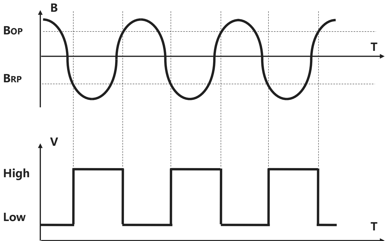
Figure.6 Digital Output vs. Magnetic Flux Density (MT8962AT as example)
